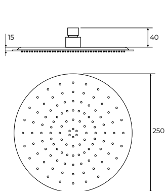
Ruža tuša Ø250mm ABS C-05-5360
