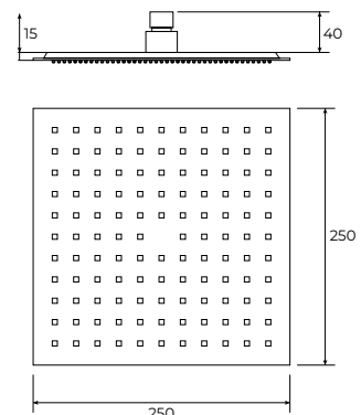
Ruža tuša 250x250mm ABS C-05-5361
